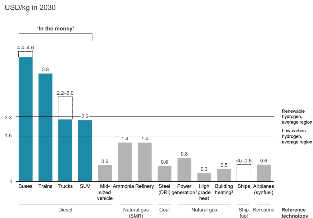
Exhibit 18: Required hydrogen production cost for breakeven with conventional solutions, without carbon costs
